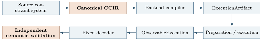
Figure 2: Simplified CPC validation architecture, adapted from the CPC Validation v0.6.0 reference framework [29].
